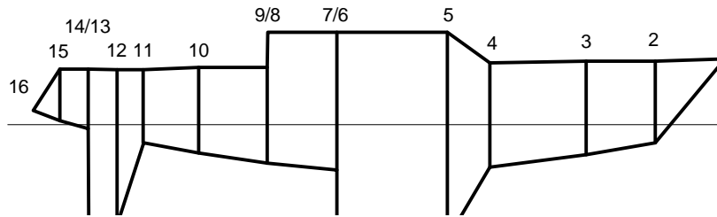
Profile of TEST25B with stations numbered.
