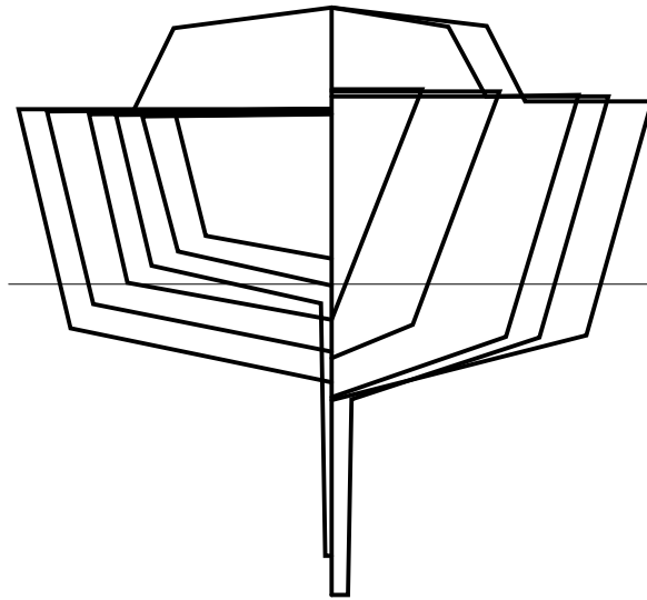
Body plan of TEST25B.
